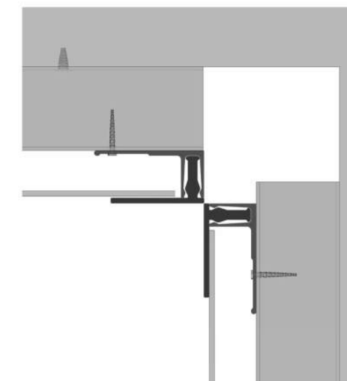
ENLARGED DETAIL B
