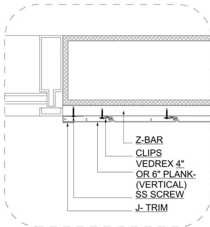
D DETAIL D-04 SCALE: 1.0" 2.0" 5.0"
