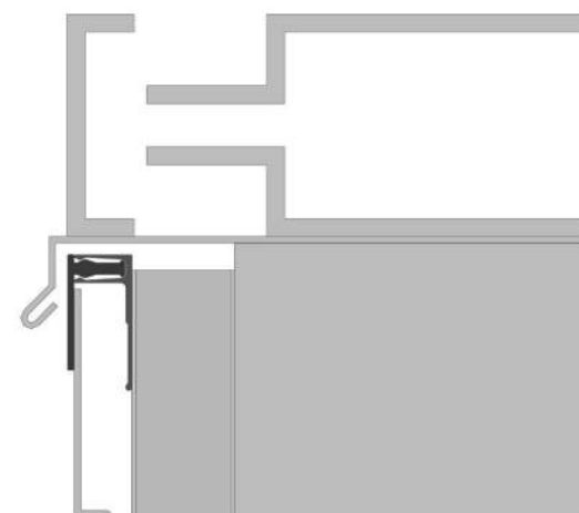
ENLARGED DETAIL A
