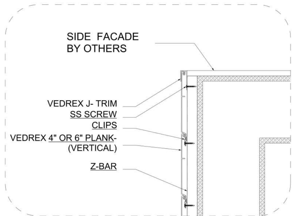
D DETAIL D-01 SCALE: 1.0" 2.0" 5.0"
