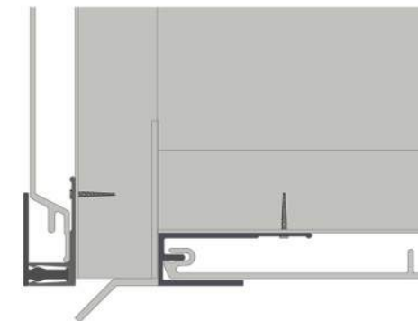
ENLARGED DETAIL B
