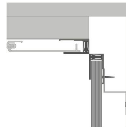
ENLARGED DETAIL C
