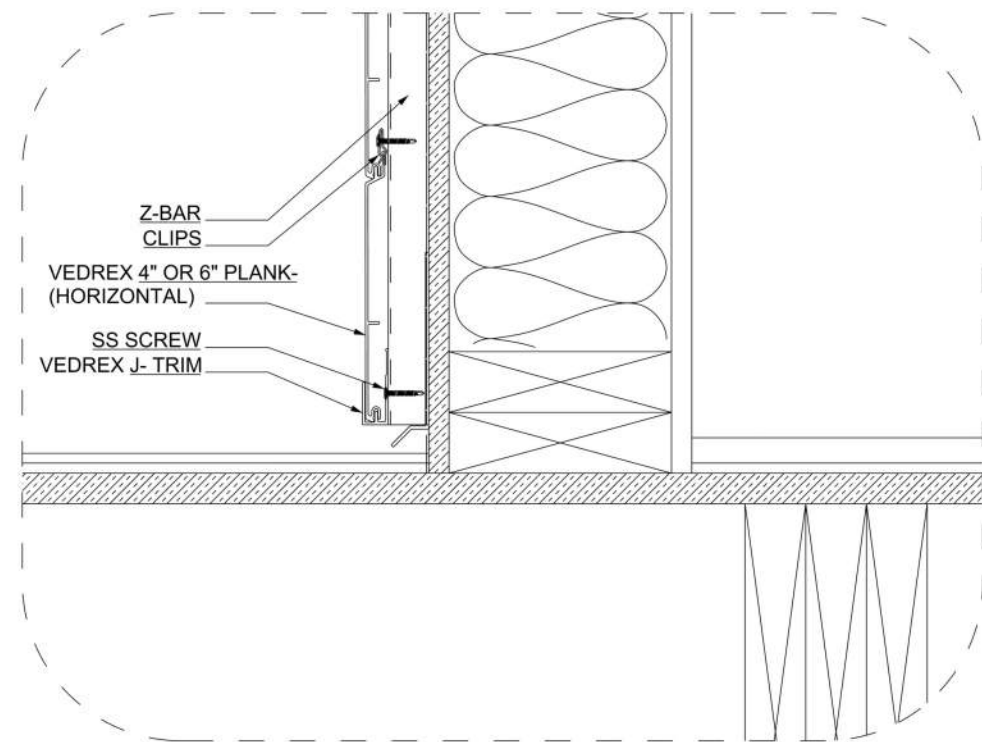
D DETAIL S-04
