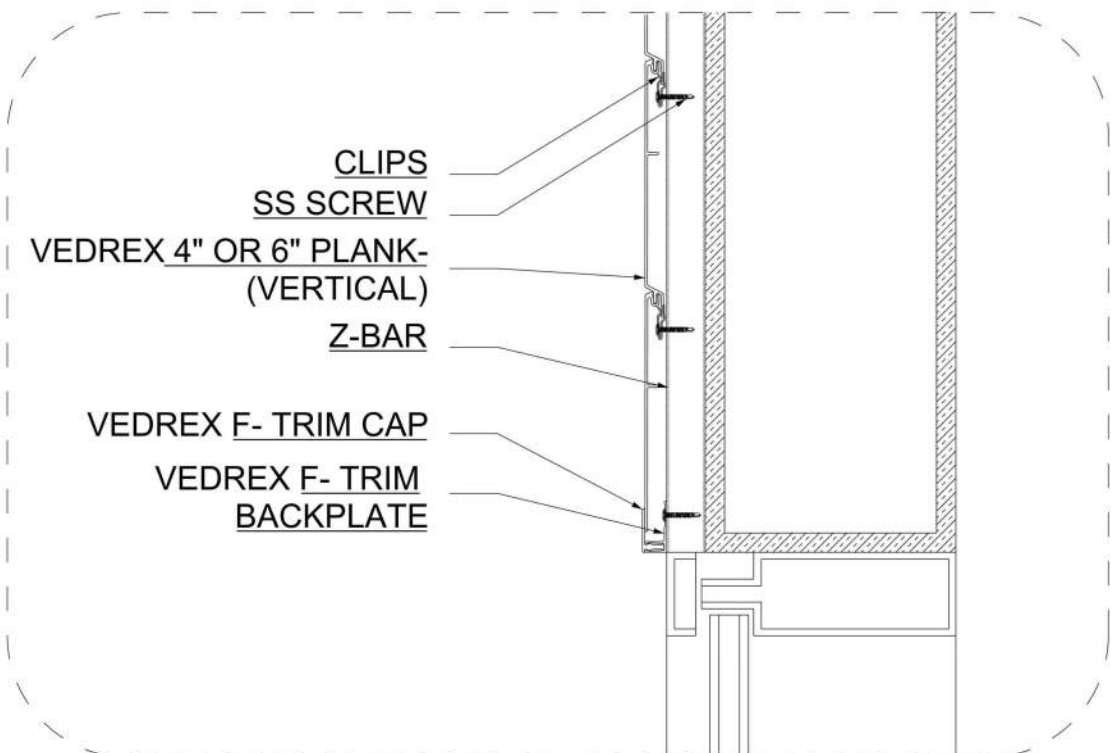
D DETAIL D-02 SCALE: 1.0" 2.0" 5.0"
