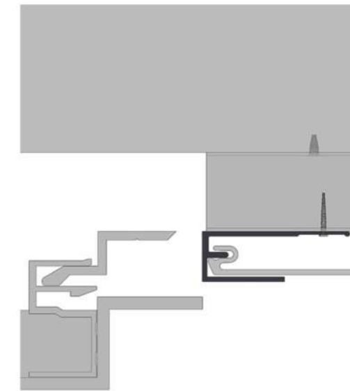
ENLARGED DETAIL A
