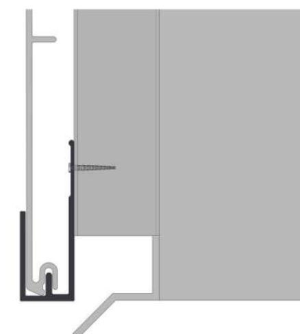
ENLARGED DETAIL C
