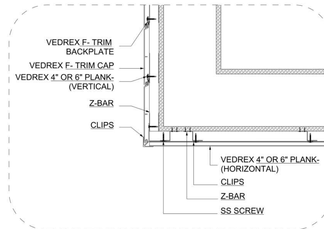
D DETAIL D-06 SCALE: 1.0" 2.0" 5.0"
