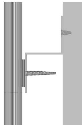
ENLARGED DETAIL B
