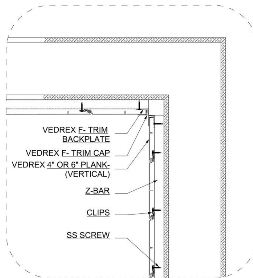
D DETAIL D-05 SCALE: 1.0" 2.0" 5.0"
