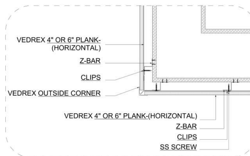
D DETAIL D-12 SCALE: 1.0" 2.0" 5.0"
