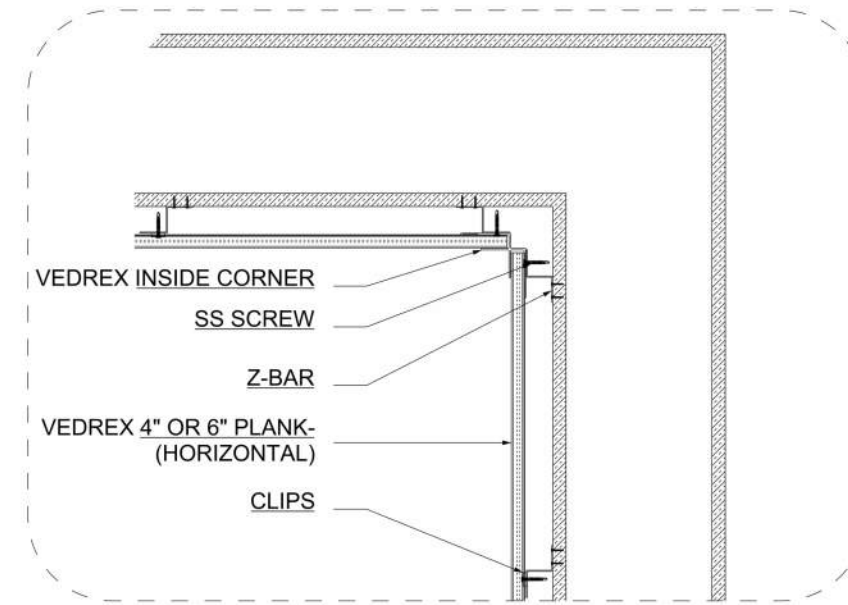
D DETAIL D-10 SCALE: 1.0" 2.0" 5.0"
