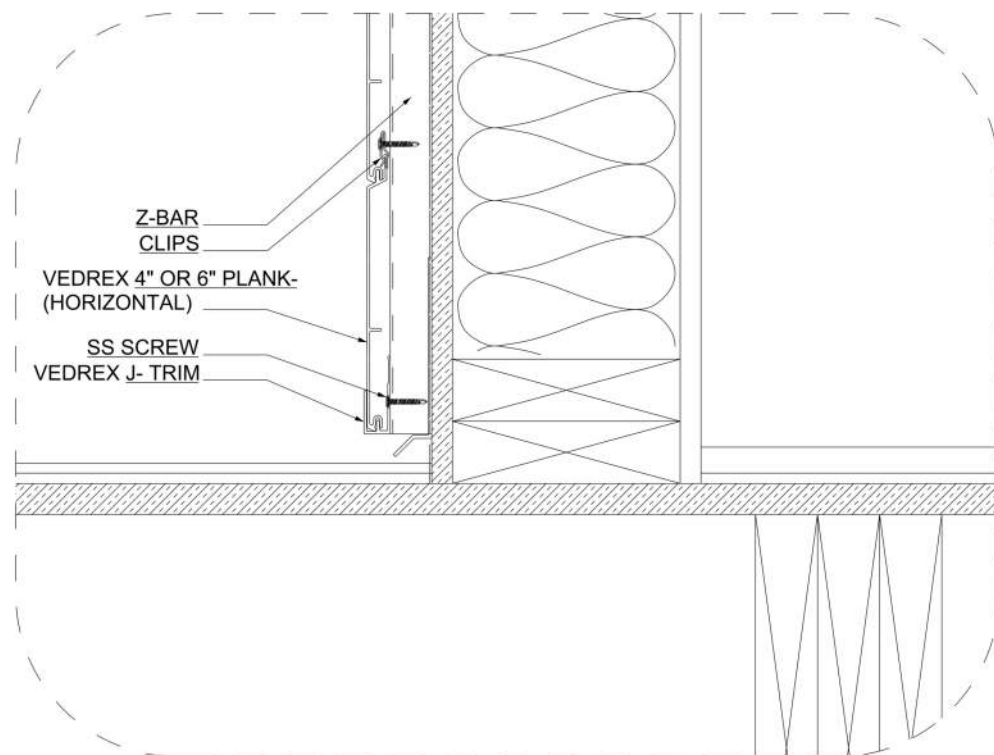
D DETAIL S-05
