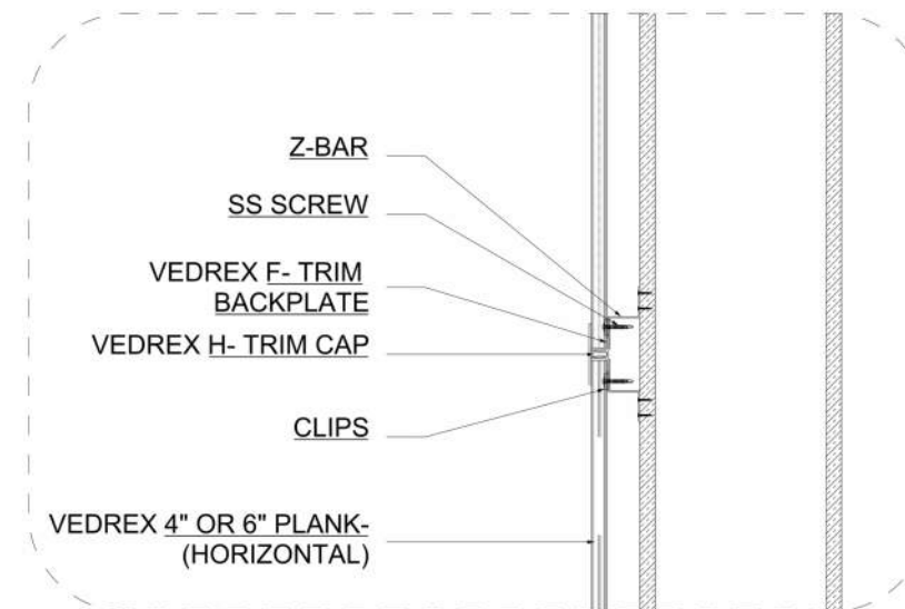
D DETAIL D-11 SCALE: 1.0" 2.0" 5.0"
